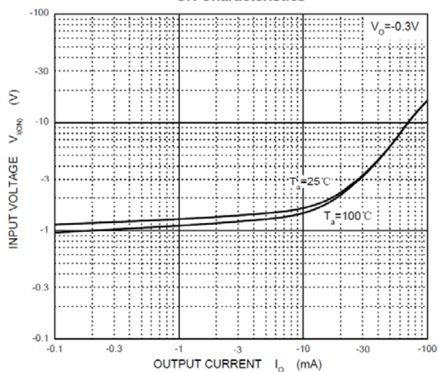
ON Characteristics
