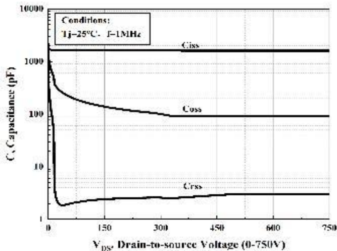
Figure 13. Capacitances vs. Drain Source Voltage (0-750V)
