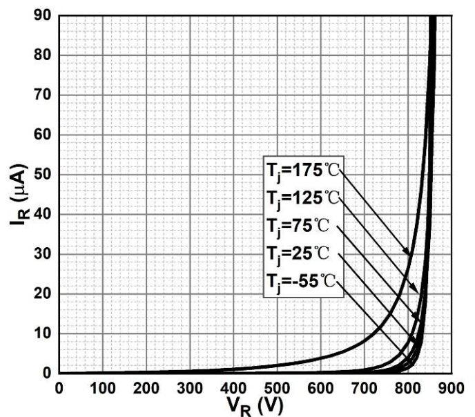
Figure 2. Reverse Characteristics
