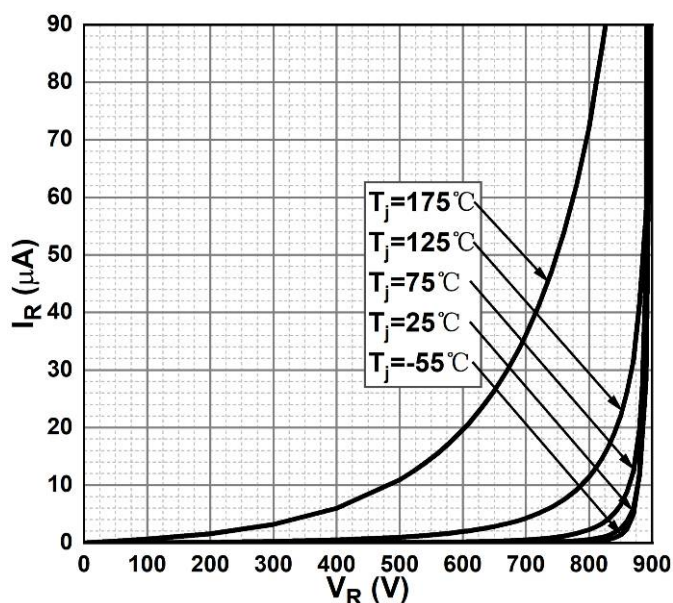
Figure 2. Reverse Characteristic
