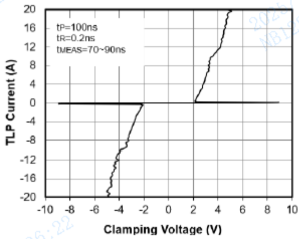
Fig5, TLP Measurement
